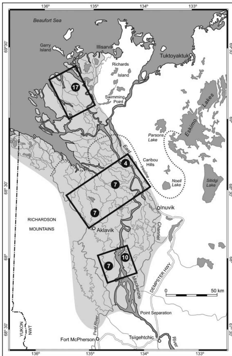
Figure 1 The Mackenzie Delta area. Permafrost in the delta is classified as discontinuous permafrost, whereas the uplands surrounding the delta are in the continuous permafrost zone (Heginbottom et al. , 1995). Field investigations were clustered in six areas with the number of sites studied in each area appearing inside the circles. The extent of the satellite images is indicated by the rectangles. Treeline is indicated by a dotted line.
