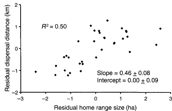
FIG. 2. Relationship between residuals of maximum natal dispersal distance (after effects of body size are removed) and residuals of home range area (after effects of body size are removed) for 34 North American mammal species. All variables are on a \log_{10} scale. Slope and intercept are expressed as mean \pm 1 SE.
