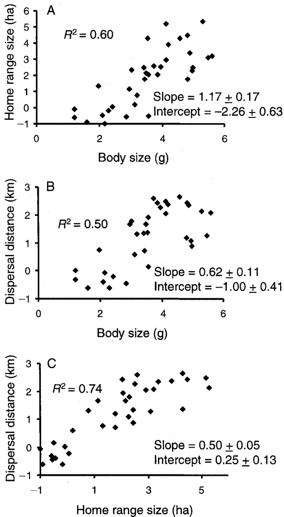
FIG. 1. Relationships between (A) home range area and body size, (B) maximum natal dispersal distance and body size, and (C) maximum natal dispersal distance and home range area for 34 North American mammal species. All variables are on a \log_{10} scale. Slope and intercept values are expressed as mean \pm 1 SE.
