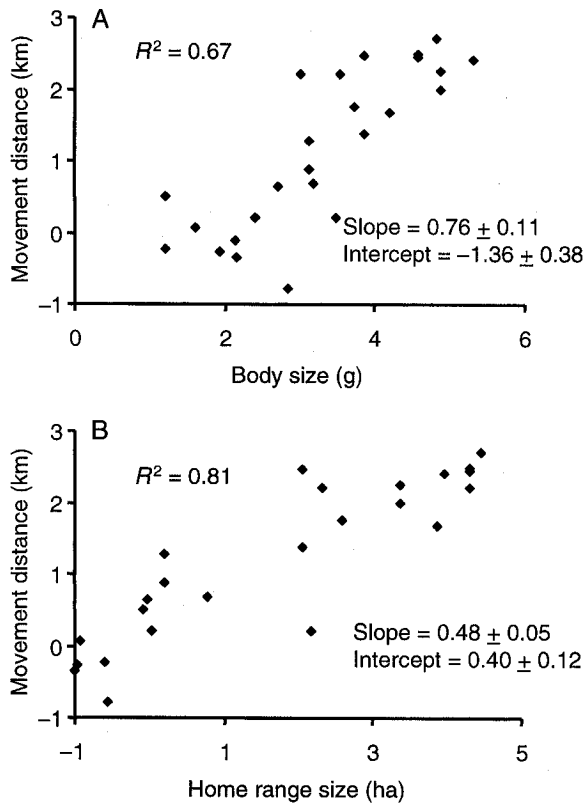
FIG. 3. Relationships (A) between maximum distance moved after translocation and body size, and (B) between maximum distance moved after translocation and home range area ( n = 25 ). All variables are on a \log_{10} scale. Slope and intercept are expressed as mean \pm 1 SE.
