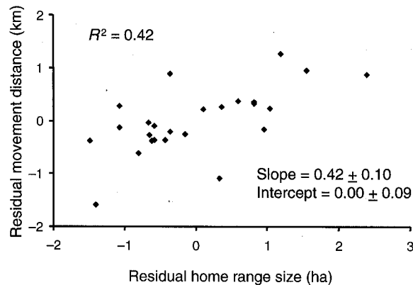
FIG. 4. Relationship between residuals of maximum distance moved after translocation (with effects of body size removed) and residuals of home range area (with effects of body size removed); n = 25 . All variables are on a \log_{10} scale. Slope and intercept are expressed as mean \pm 1 SE.
